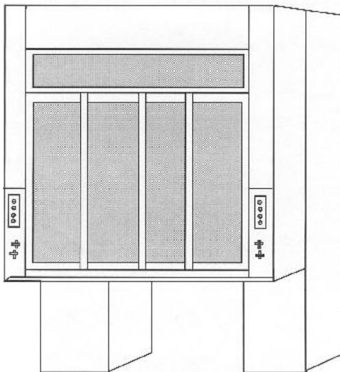
Figure 3.20 A simplified version of a horizontal sash hood that complies with the provisions of the Americans with Disabilities Act. The space between the two pedestals is wide enough and high enough to accommodate an individual in a wheel chair. When this feature is not needed, a storage cabinet may be put in this space. The pedestals are also usable for storage.
