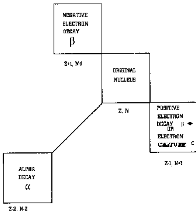
Figure 5.1 Schematic representation of the decay process.
