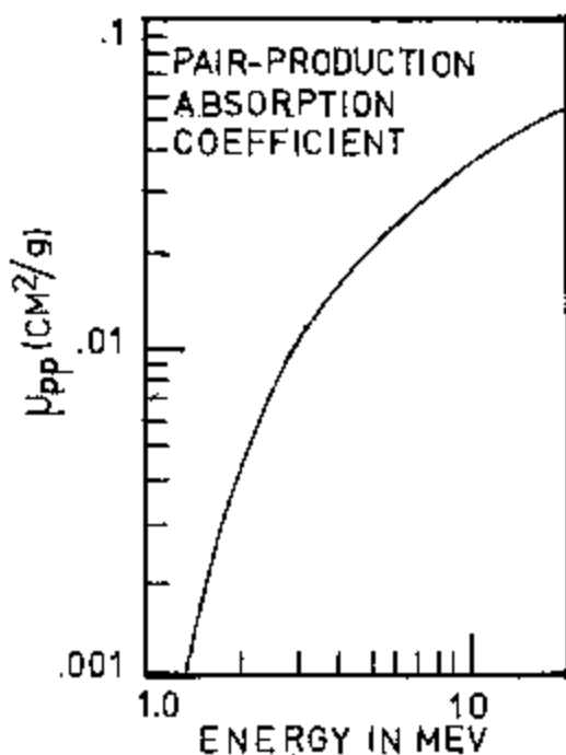
Figure 5.4 Pair-production coefficient for lead as a function of energy.
