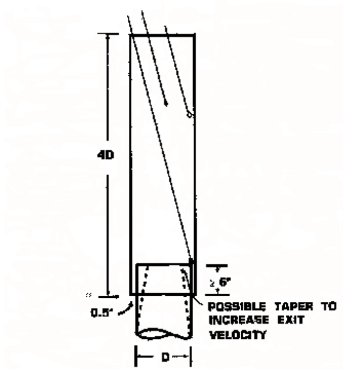
Figure 3.23 Exhaust duct rain shield.
