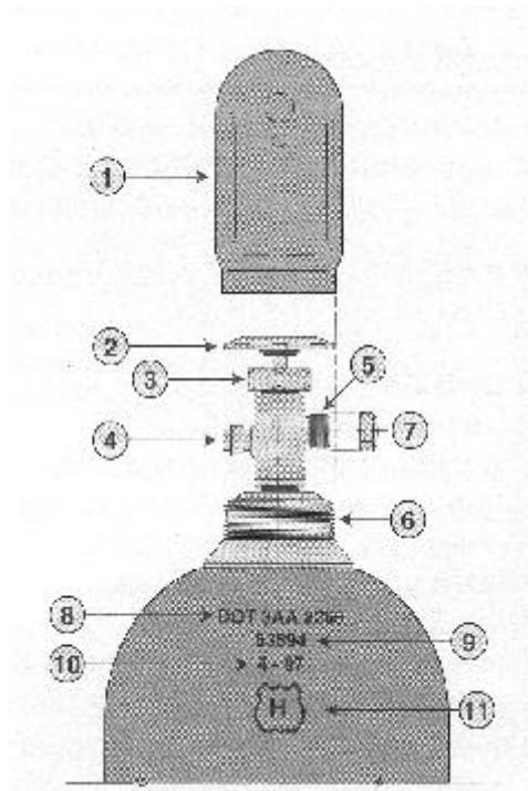
Figure 4.3 Cylinder parts and markings, (1) cylinder cap; (2) cylinder valve wheel to open cylinder; (3) valve packing nut, contains a packing gland and packing nut around the valve stem; (4) pressure relief device; (5) valve outlet connection; (6) cylinder collar to which cap is to be attached; (7) valve outlet cap, may not be present; (8) Specification number shows cylinder conforms to DOT-3AA specifications; and design service pressure is 2265 psig @ 70°F; (9) indicates date, month and year first tested. Test is to be repeated every 5 years and test date stamped on cylinder. This figure and Figures 4.4 and 4.5 courtesy of Matheson Gas Products.
