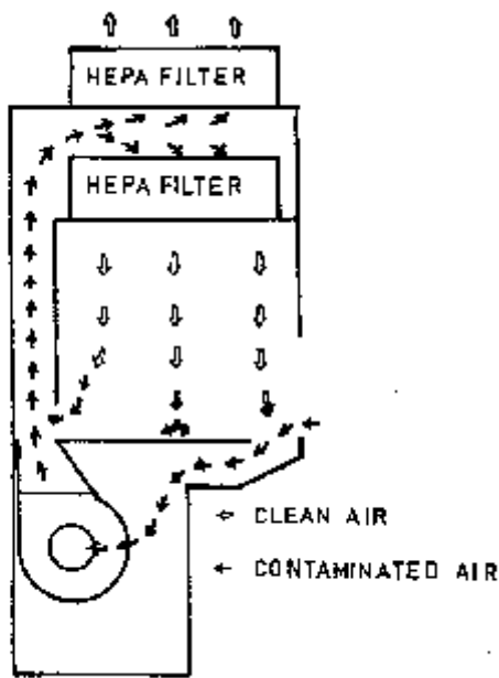
Figure 3.26 Class II biosafety cabinet.
