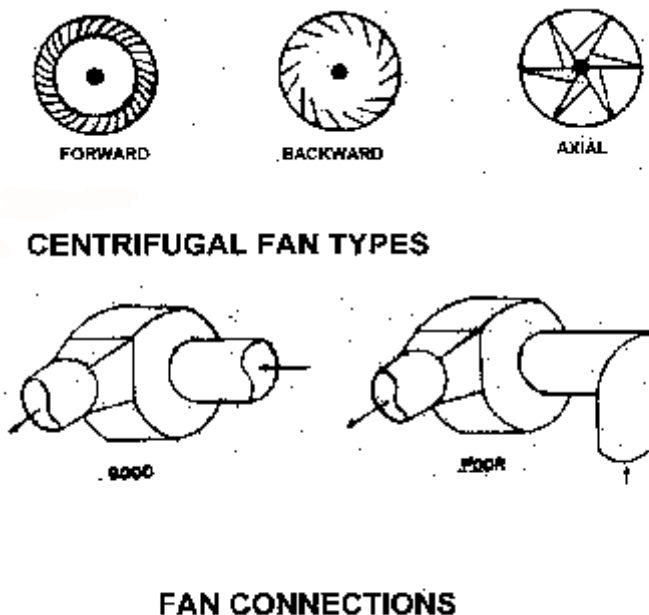
Figure 3.24 (Top) Types of centrifugal fan designs. (Bottom) Exhaust duct fan connections.
