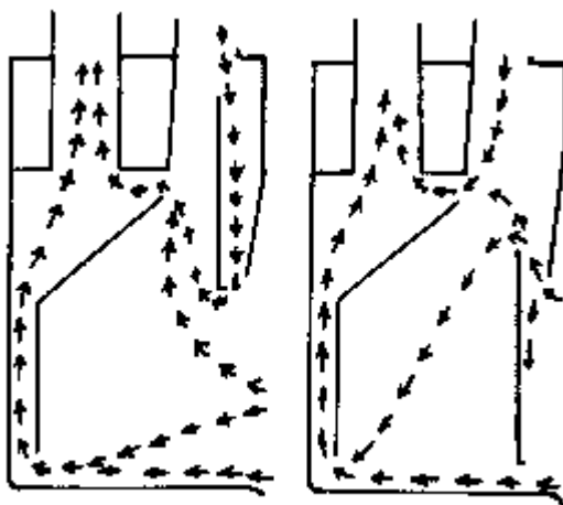
Figure 3.18 Auxiliary or add-air hood, sash open and closed.
