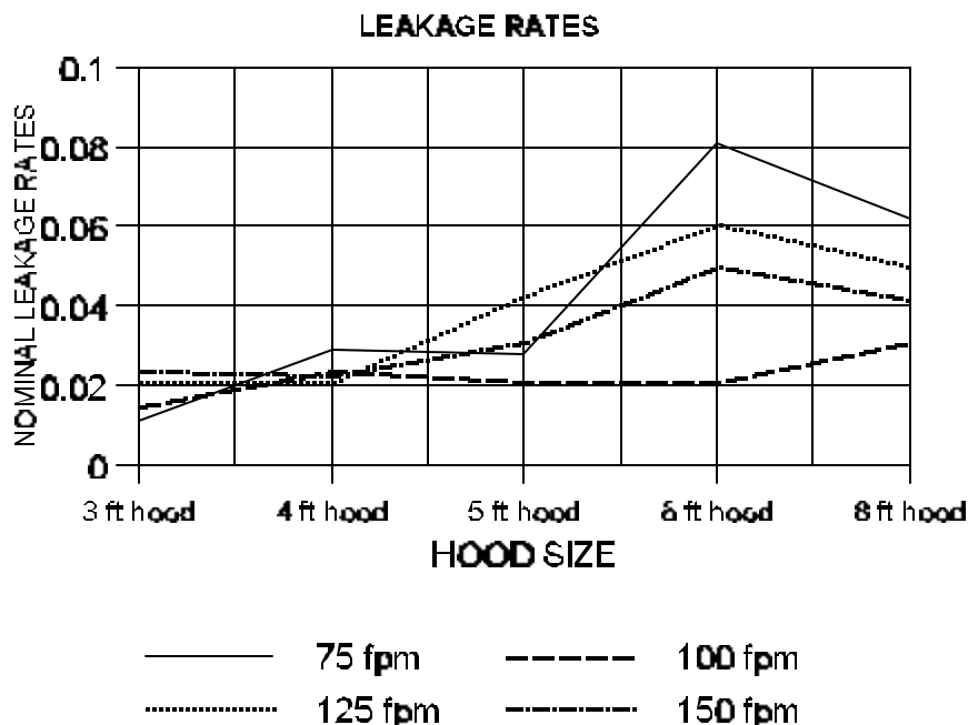
Figure 3.12 Leakage rates for various face velocities for different size bench hoods. The rates are not absolute but are values in ppm for the experimental challenge rate for the contaminant gas.
