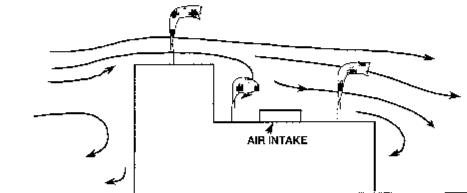
Figure 3.7 Effect of building shape on wind flow in its vicinity.
