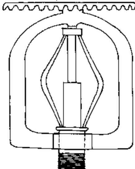
Figure 3.29 Upright sprinkler head.
