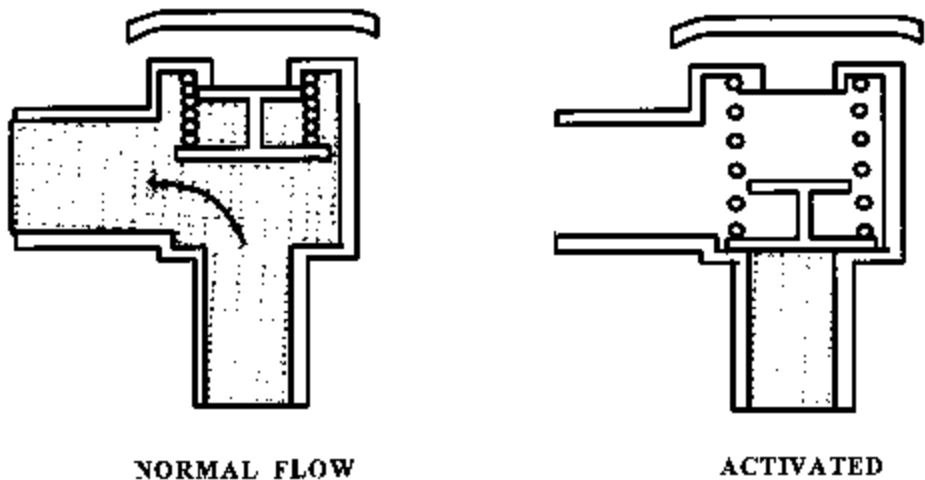
Figure 3.9 Vacuum breaker.
