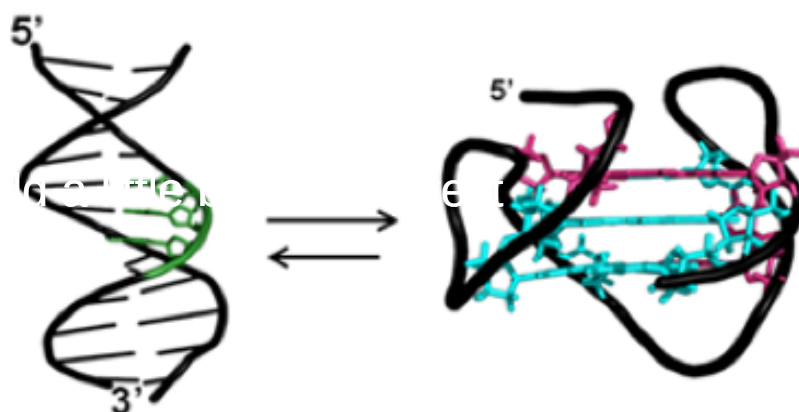
Watson-Crick Duplex DNA
